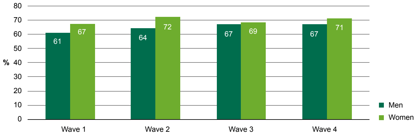
Figure 2.1 IRP scores by gender (Waves 1–4)
